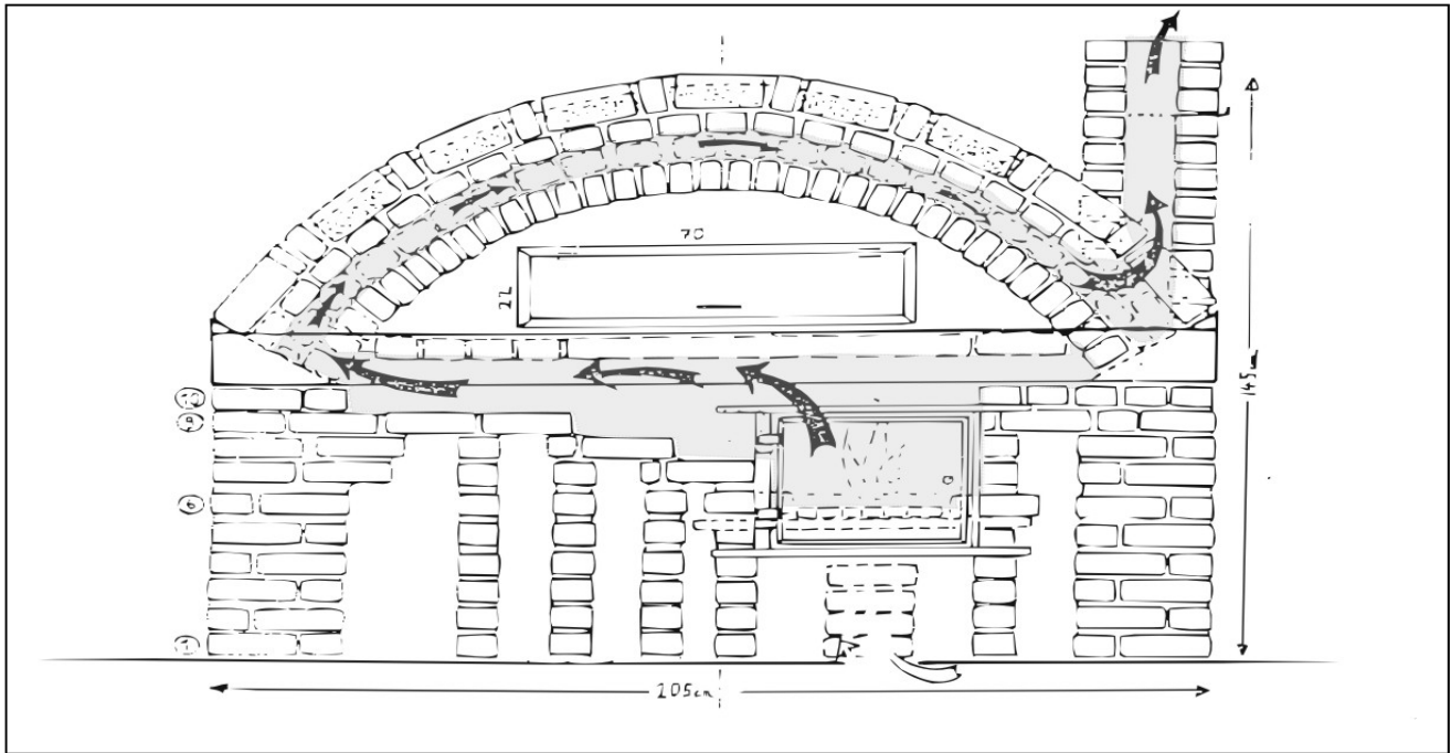
MFBO - Multi Fuel Bread Oven from Burundi / East Africa
