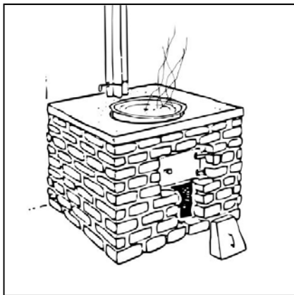
US-AID/ Burundi Community Stove
